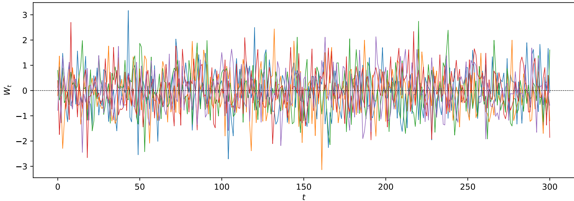
White Noise W_t \stackrel{\text{i.i.d.}}{\sim} \mathcal{N}(0, \sigma_W^2) , \sigma_W = 0.8 , 5 realizations
